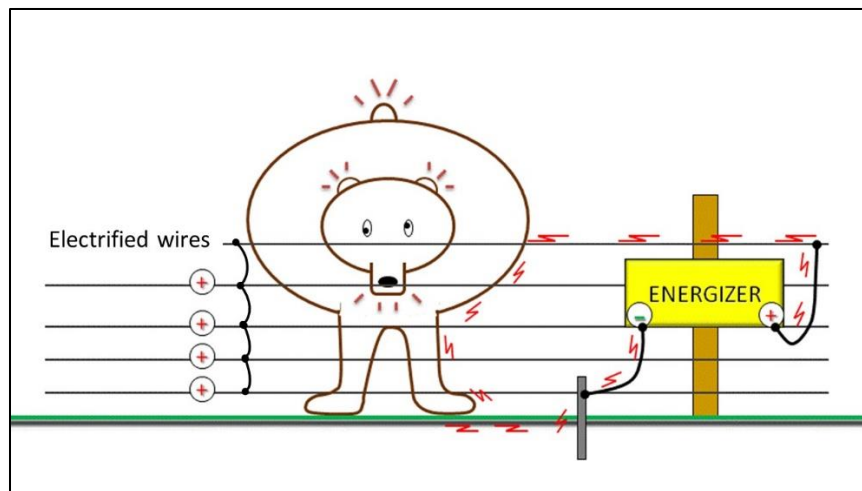
Figure 2. An all-hot electrified fence design. All wires are connected to each other in series and to the positive terminal on the energizer. The negative terminal of the energizer is connected to the grounding rod.
