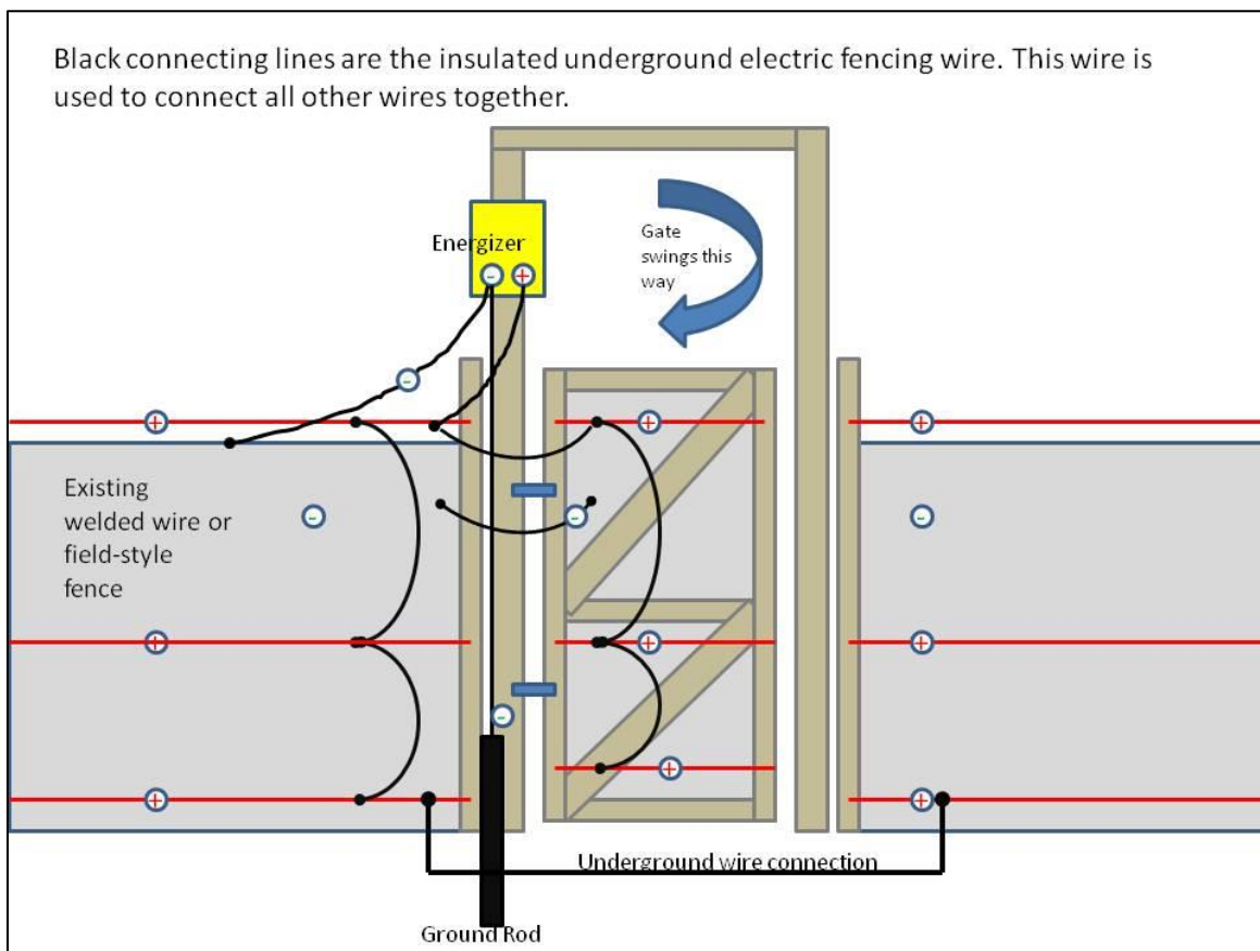
Figure 11. An example of how a gate can be electrified by attaching it to the electrified lines on the main fence, and how 2 sections of fence can be electrified with an underground wire connection.
