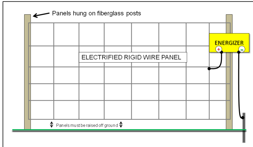
Figure 6. Electrified rigid wire panel. The panel is raised off the ground and insulated by hanging it from fiberglass posts or plastic insulators. The wire panel is electrified by connecting it directly to the positive terminal on the energizer. The ground rod is connected to the negative terminal of the energizer.
