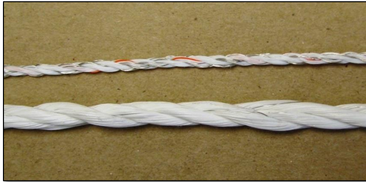
Figure 4. Two different styles of 9-stranded Polywire
