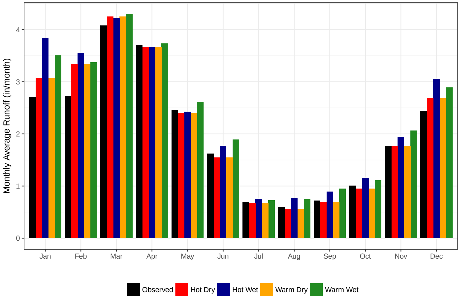
Climate Change Streamflow Projections for Salmon Regional Basin
