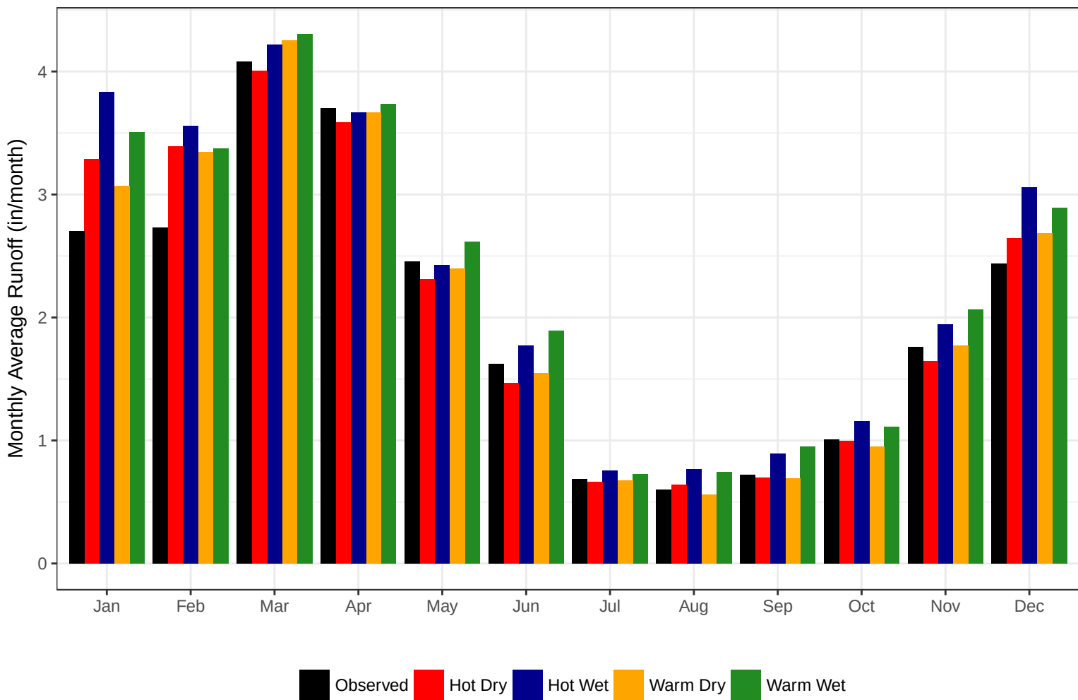
Climate Change Streamflow Projections for Yantic Regional Basin
