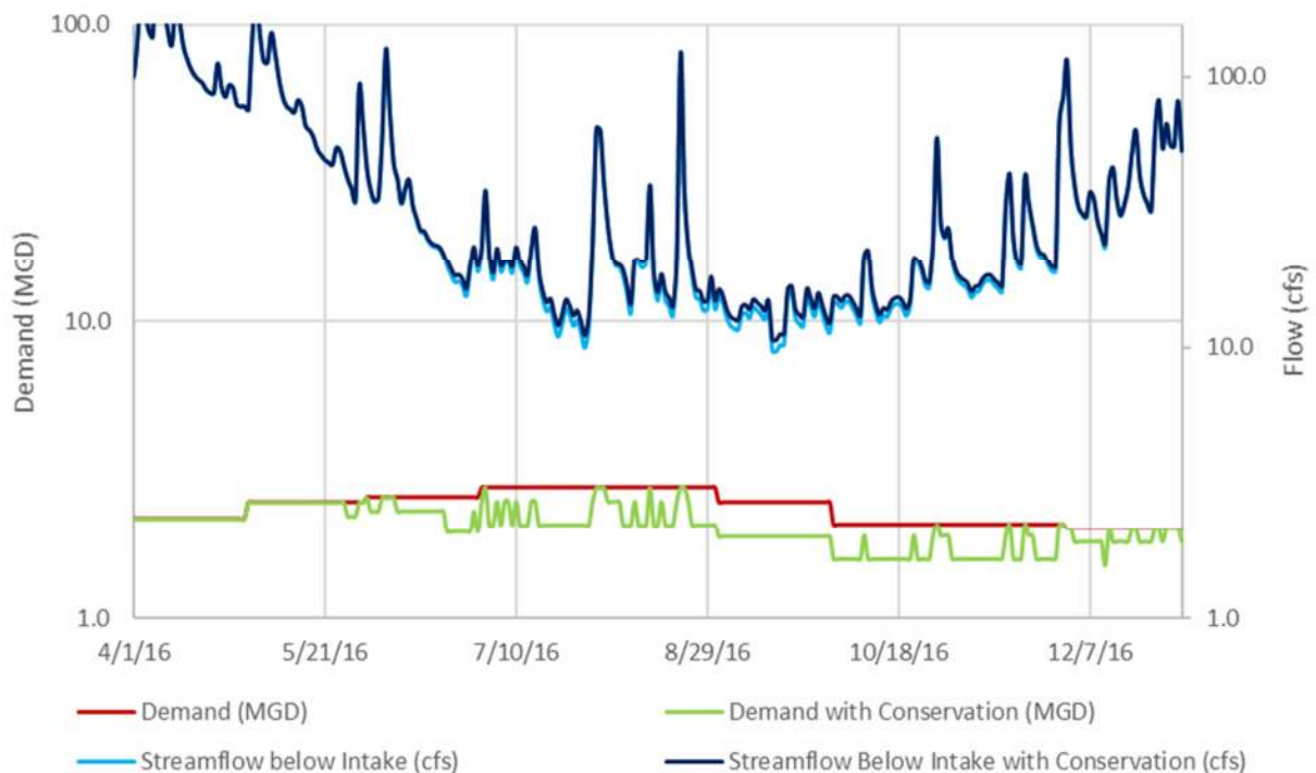
Figure 3-28. Water Conservation Example
