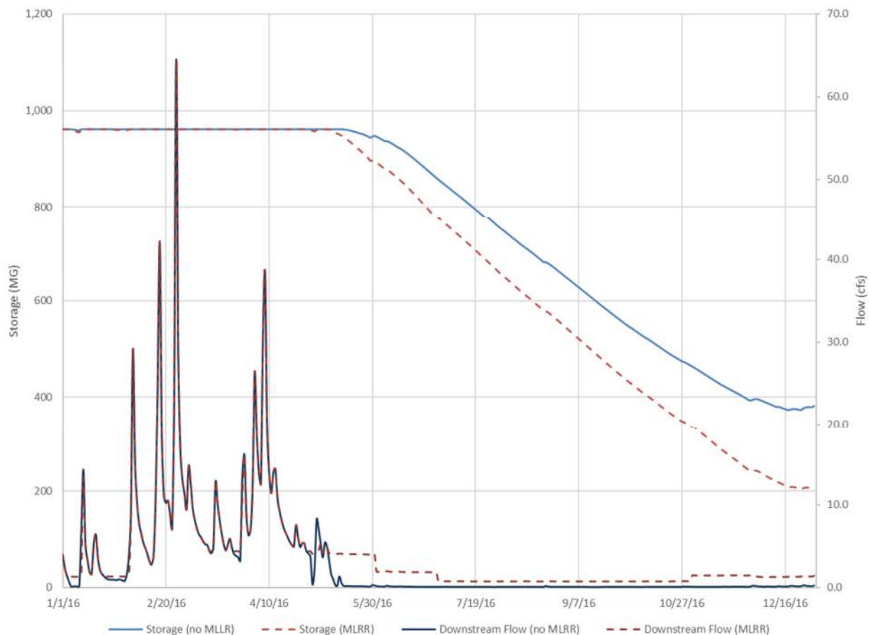
Figure 3-29. Reservoir Release Rule Example
