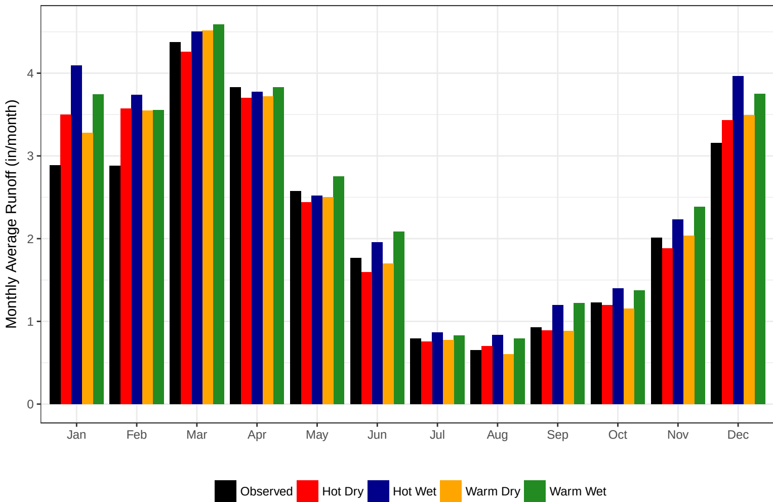
Climate Change Streamflow Projections for Candlewood Regional Basin
