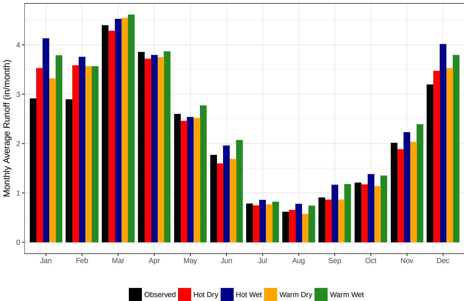
Climate Change Streamflow Projections for Saugatuck Regional Basin
