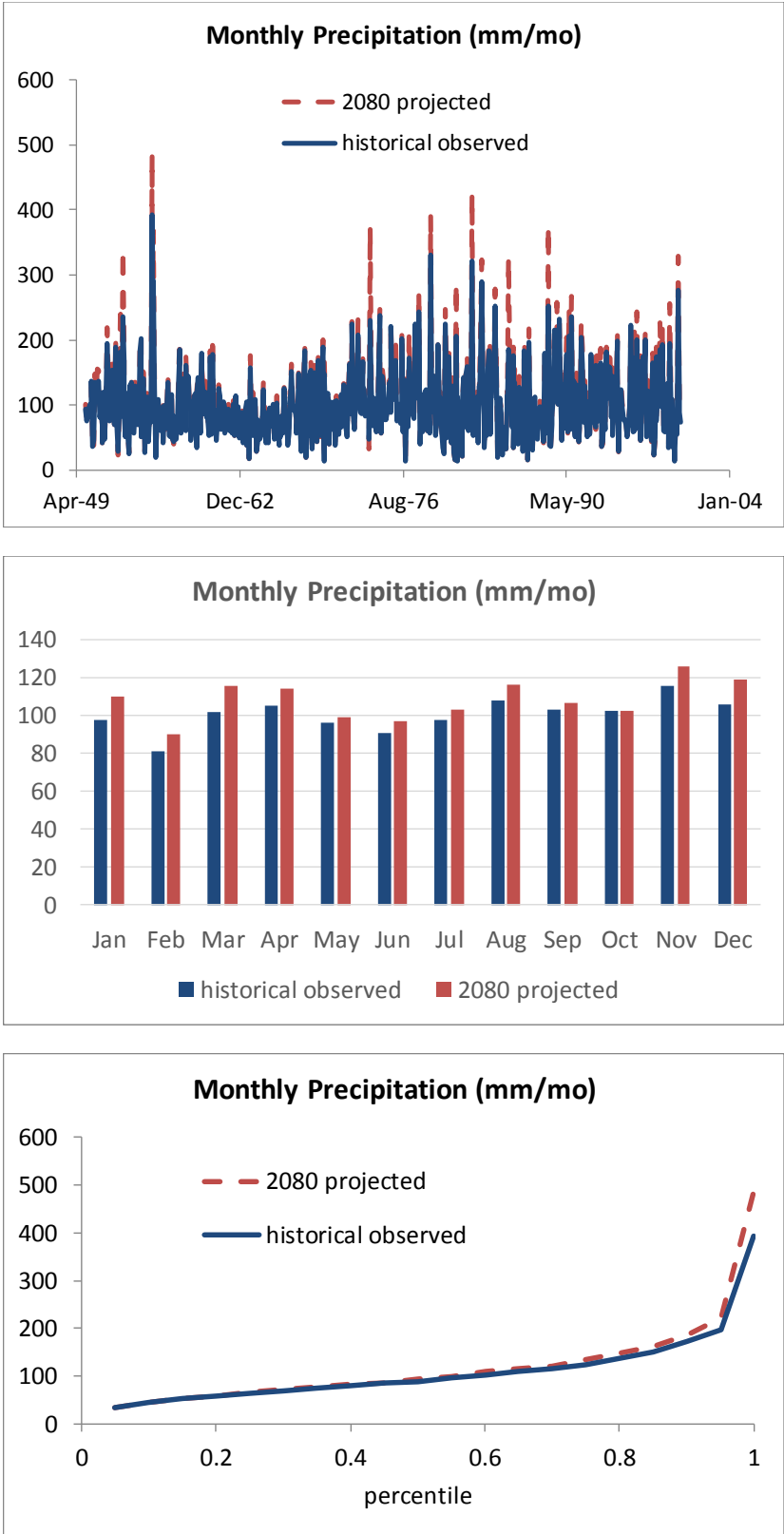
Figure 3-14. Monthly Precipitation Projections: 2080 Planning Horizon, Warm Dry Ensemble
