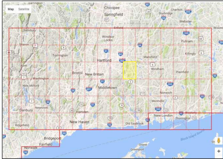
Figure 3-9. Representative Climate Model Projection Grid Cell (yellow highlight)
