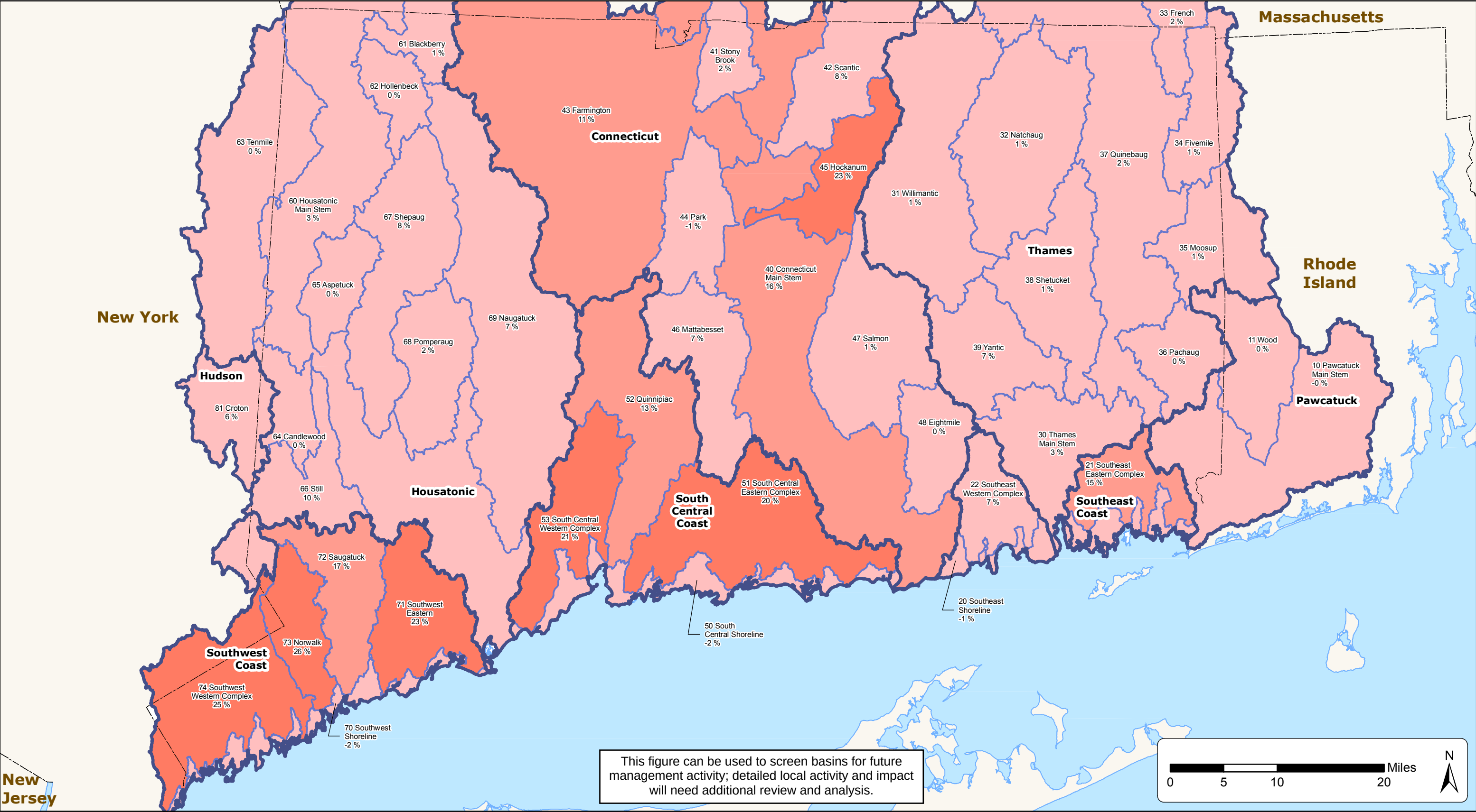
Figure 3-1 Future Out-of-stream Water Needs and Reservoir Release Requirements as a Percent of Average Annual Streamflow Connecticut State Water Plan CDM Smith MILONE & MACBROOM
