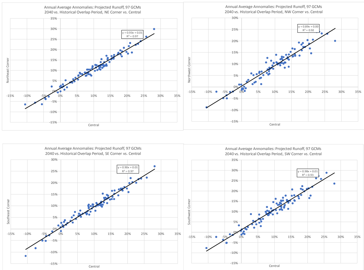
Figure 3-20. Grid Cell Comparisons: Assessment of Spatial Variability in Connecticut Gridded Runoff Projections
