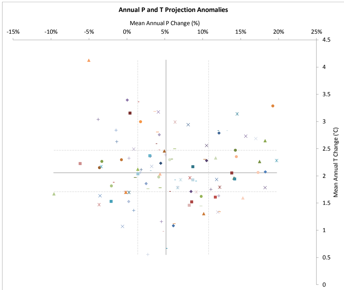
Figure 1. Example GCM Annual Anomaly Plot. Dashed grey lines indicate 25 th and 75 th percentiles. Solid grey lines indicated median values. Each symbol corresponds to a unique GCM projection.
