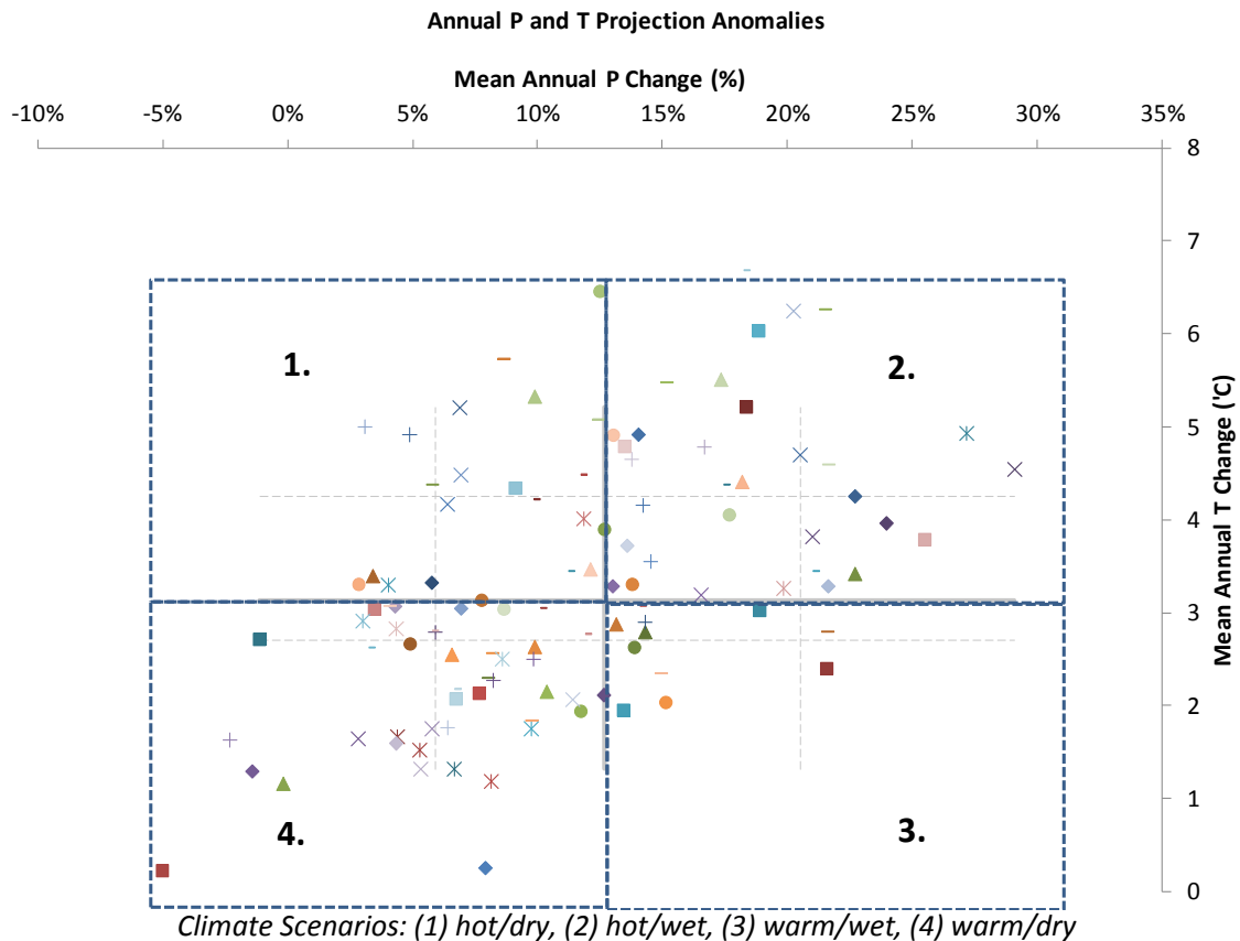
Figure 3-10. Annual Anomalies (2080 vs. historical) of GCM Temperature and Precipitation Projections, with Designated Scenario Ensembles (each symbol represents a different climate model projection set)
