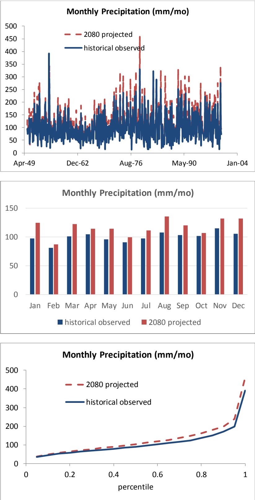
Figure 3-18. Monthly Precipitation Projections: 2080 Planning Horizon, Warm Wet Ensemble
