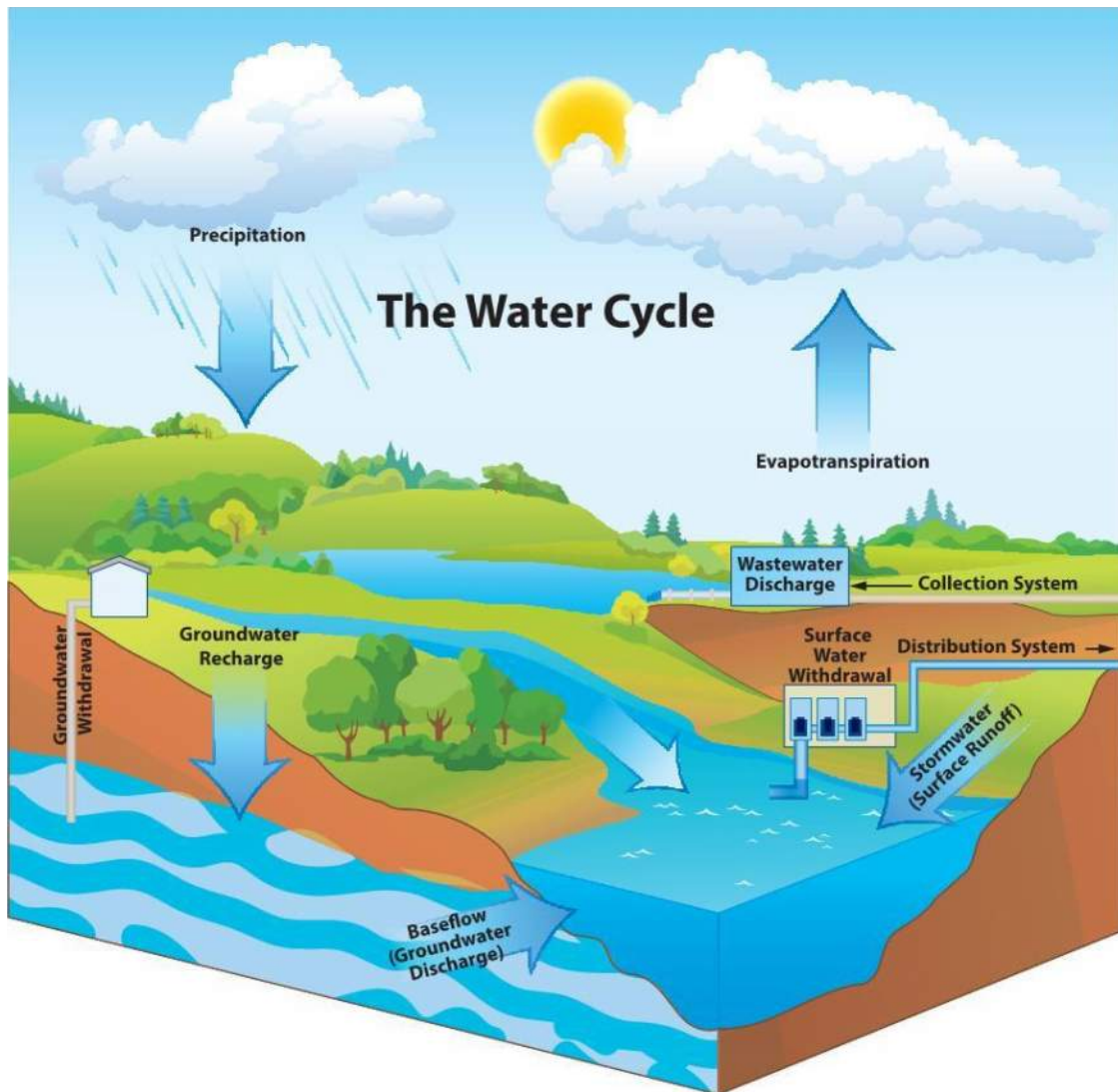
Figure 2-2. The Water Cycle
