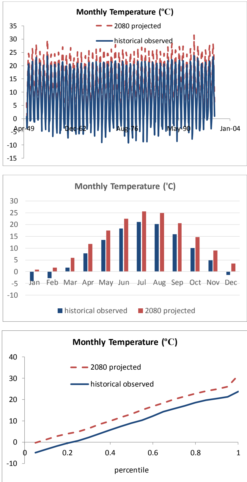
Figure 3-15. Monthly Temperature Projections: 2080 Planning Horizon, Hot Wet Ensemble
