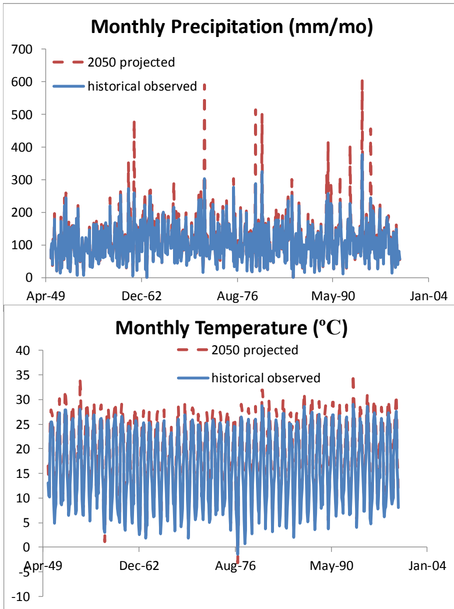
Figure 2. Example Final HDe Output: Adjusted Climate Timeseries. 2050 Planning Horizon
