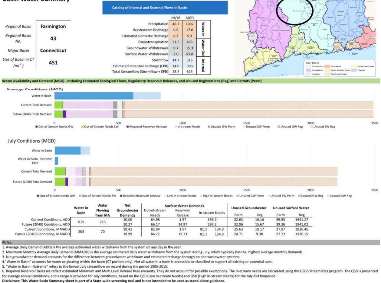
Figure 3-7. Basin Water Summary Sheet of the Farmington Regional Basin (Shown as an example – the full set of Summary Sheets for all 44 basins is included as Appendix E)
