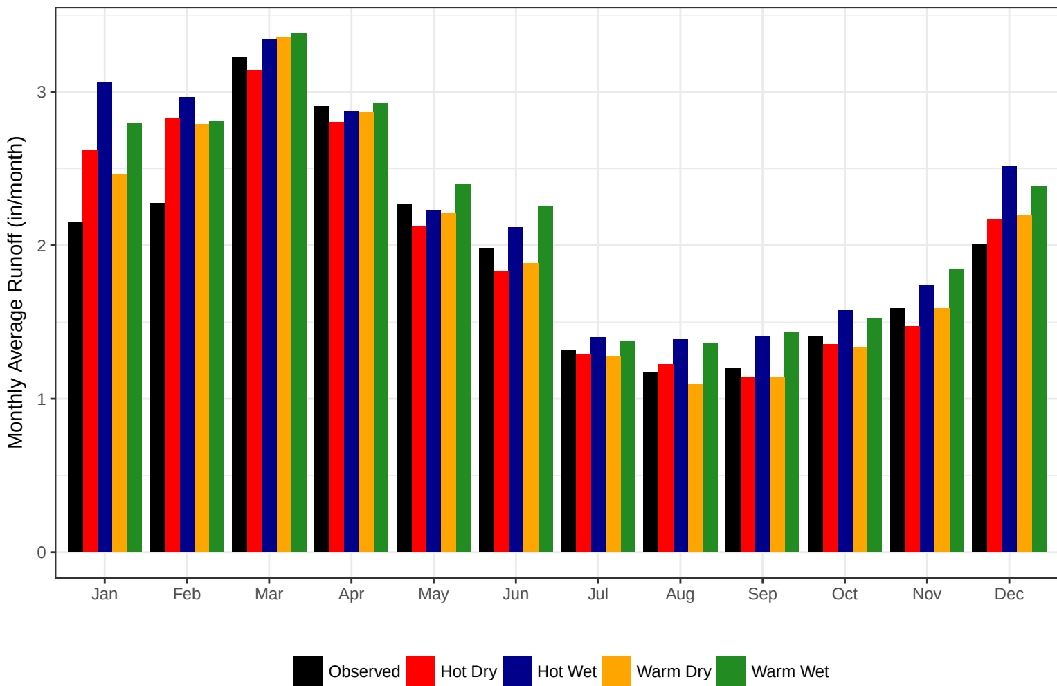
Climate Change Streamflow Projections for Scantic Regional Basin
