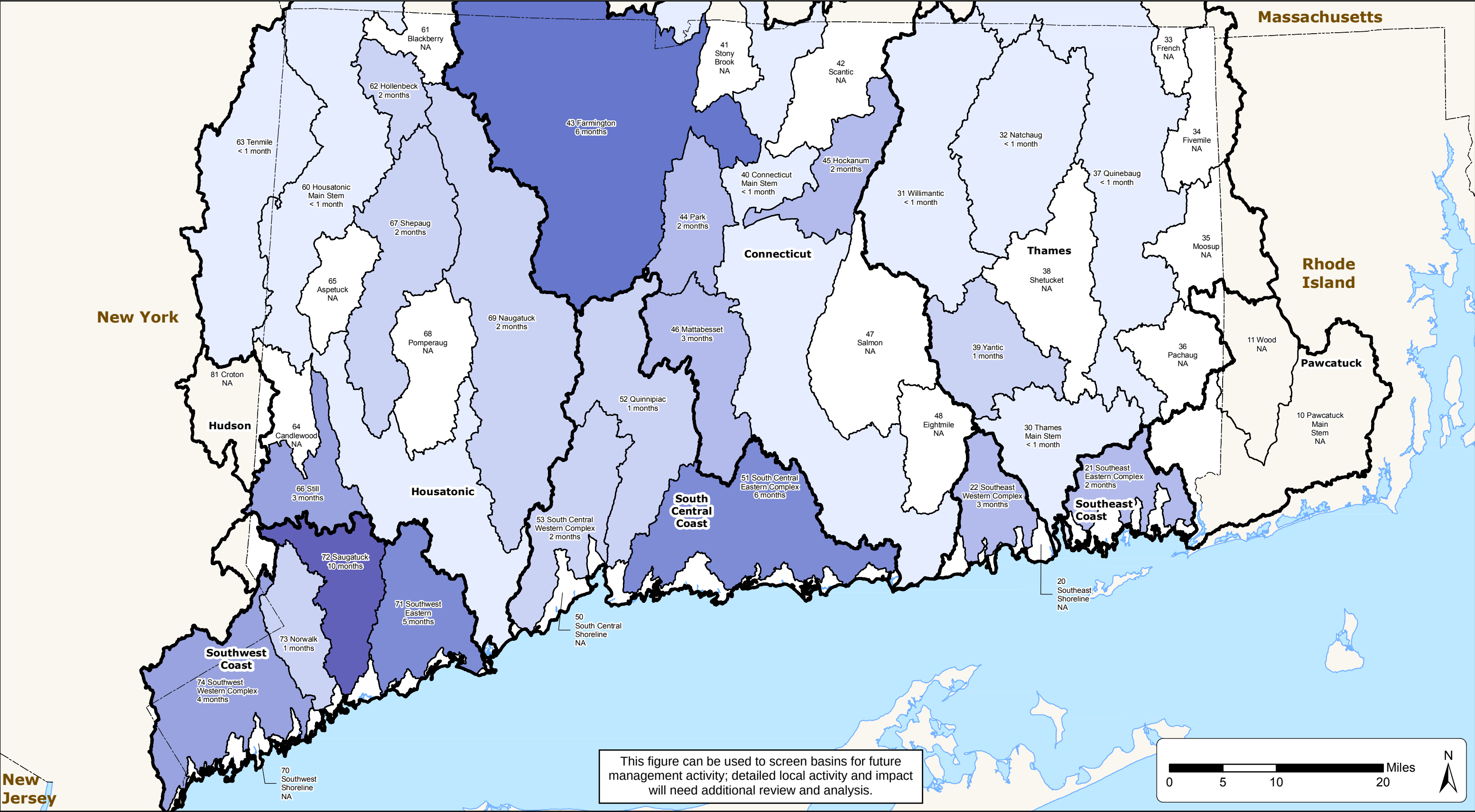
Figure 3-6 Months of Usable Storage at Future Average July Out-of-stream and In-stream Water Demand Connecticut State Water Plan
