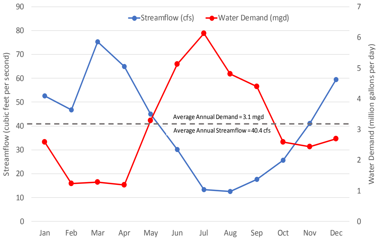
Figure 2-7. Comparison of Typical Seasonal Variations in Streamflow and Water Demand
