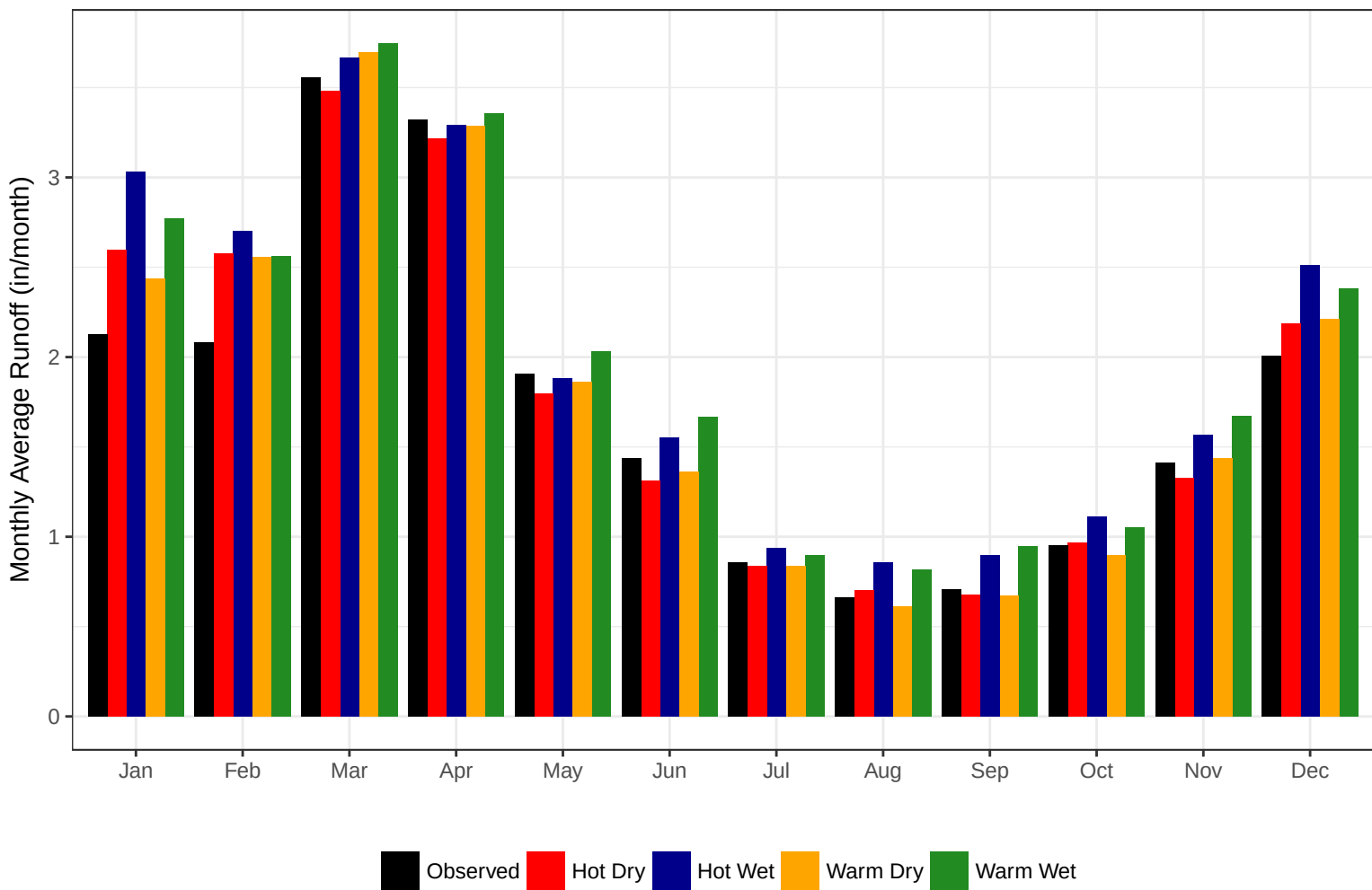
Climate Change Streamflow Projections for Tenmile Regional Basin
