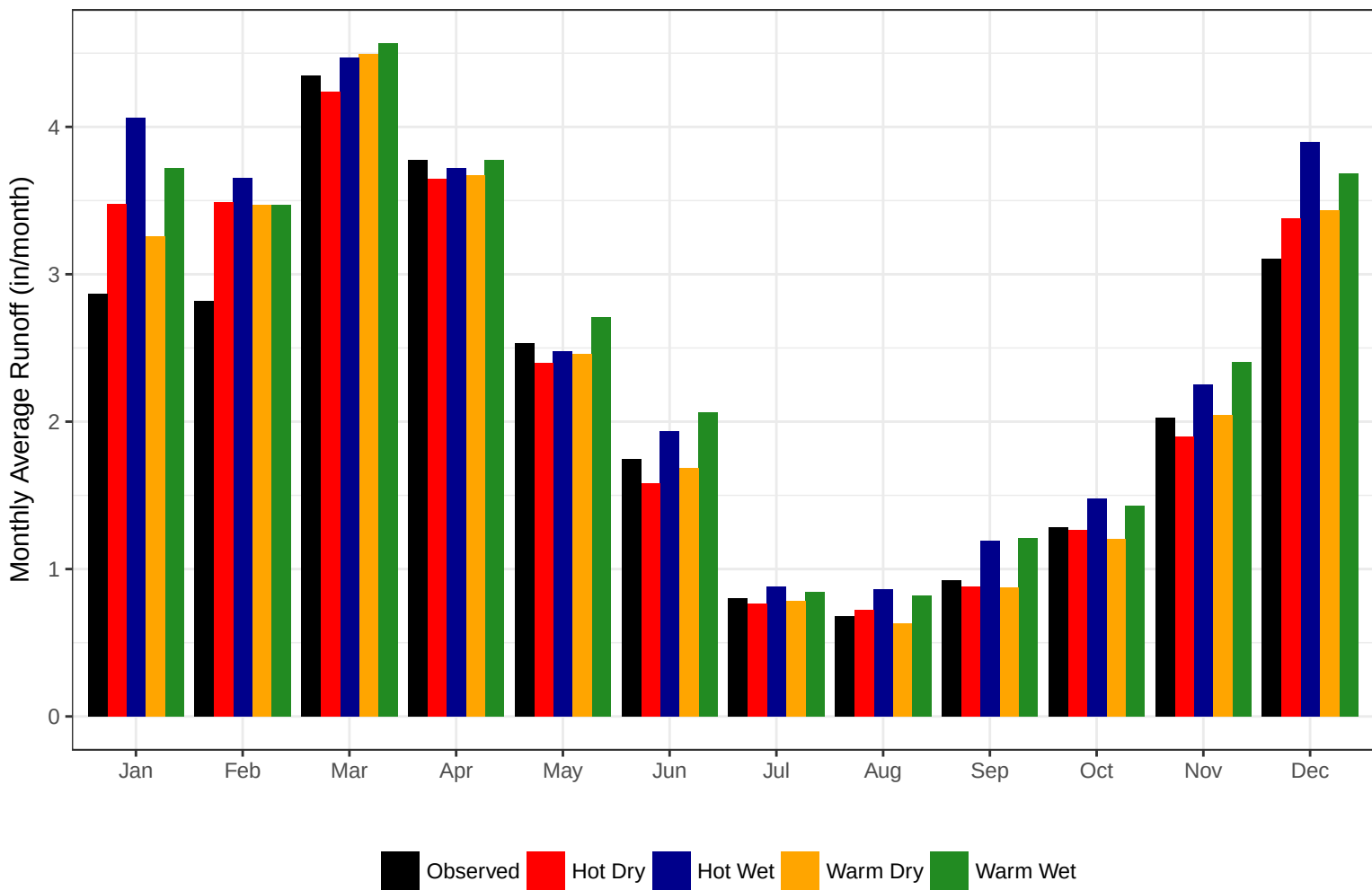
Climate Change Streamflow Projections for Croton Regional Basin
