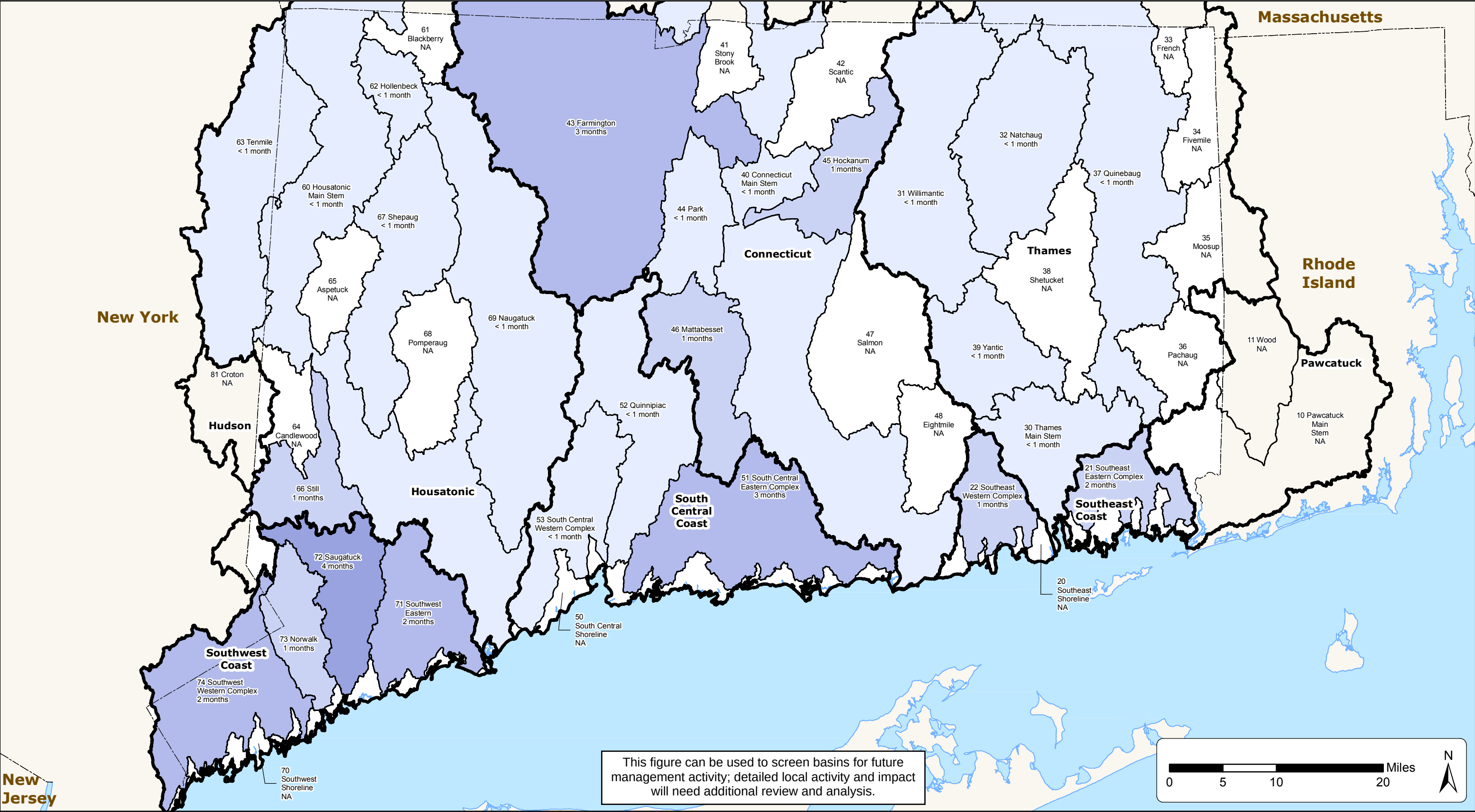
Figure 3-5 Months of Usable Storage at Future Average Annual Out-of-stream and In-stream Water Demand Connecticut State Water Plan CDM Smith MILONE & MACBROOM®
