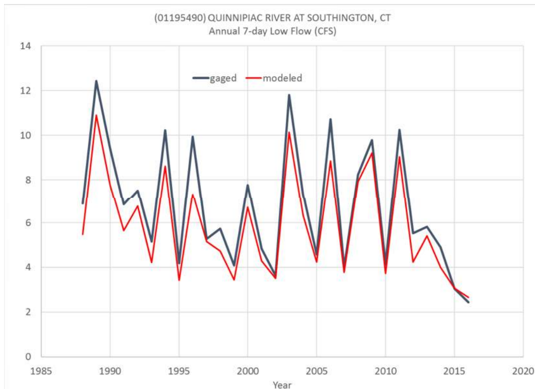
Figure 3-27. Low Flows. 7-day Annual Low Flows
