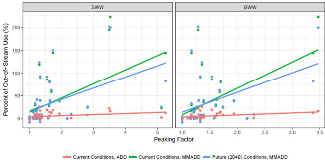
Figure 3-24. Statistically-Significant ( p < 0.05 ) Correlations of Peaking Factor and Out-of-Stream Water Use for Current and Future Average (ADD) and Monthly Maximum (MMADD) Conditions
