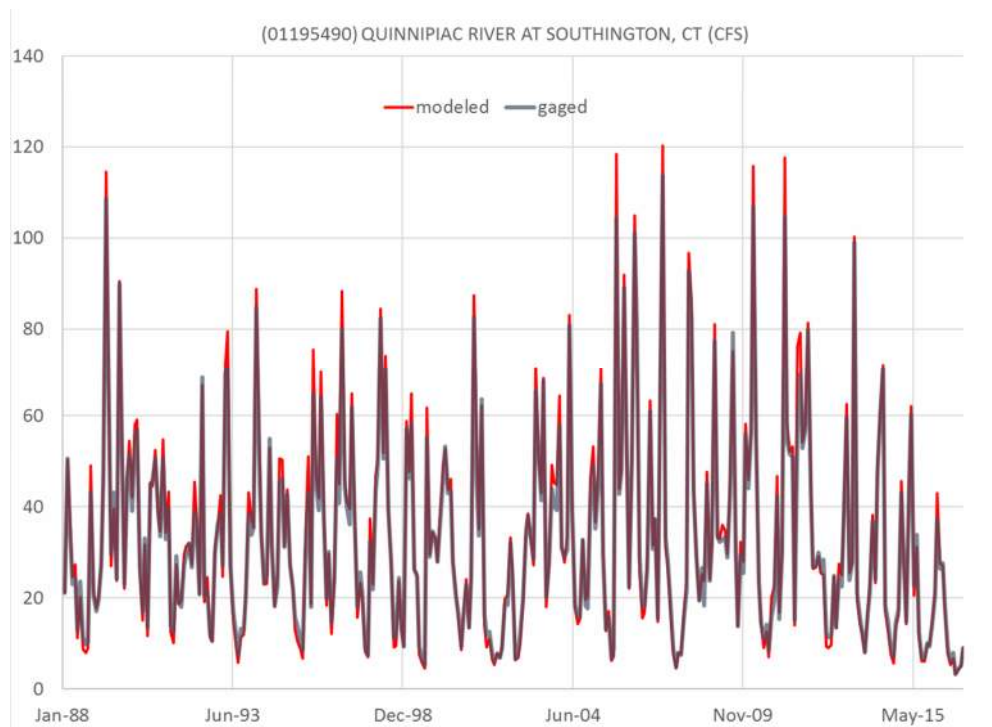
Figure 3-26. Modeled and Measured Monthly Average Streamflow
