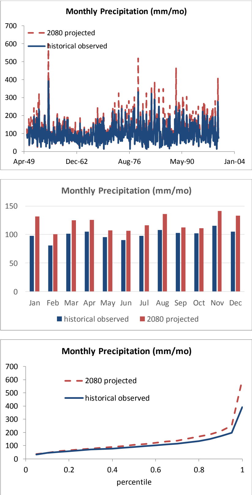
Figure 3-16. Monthly Precipitation Projections: 2080 Planning Horizon, Hot Wet Ensemble
