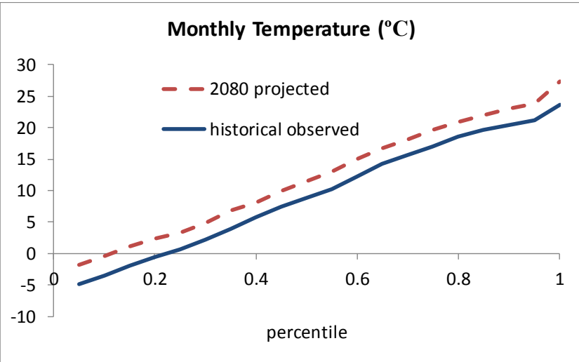
Figure 3-17. Monthly Temperature Projections: 2080 Planning Horizon, Warm Wet Ensemble
