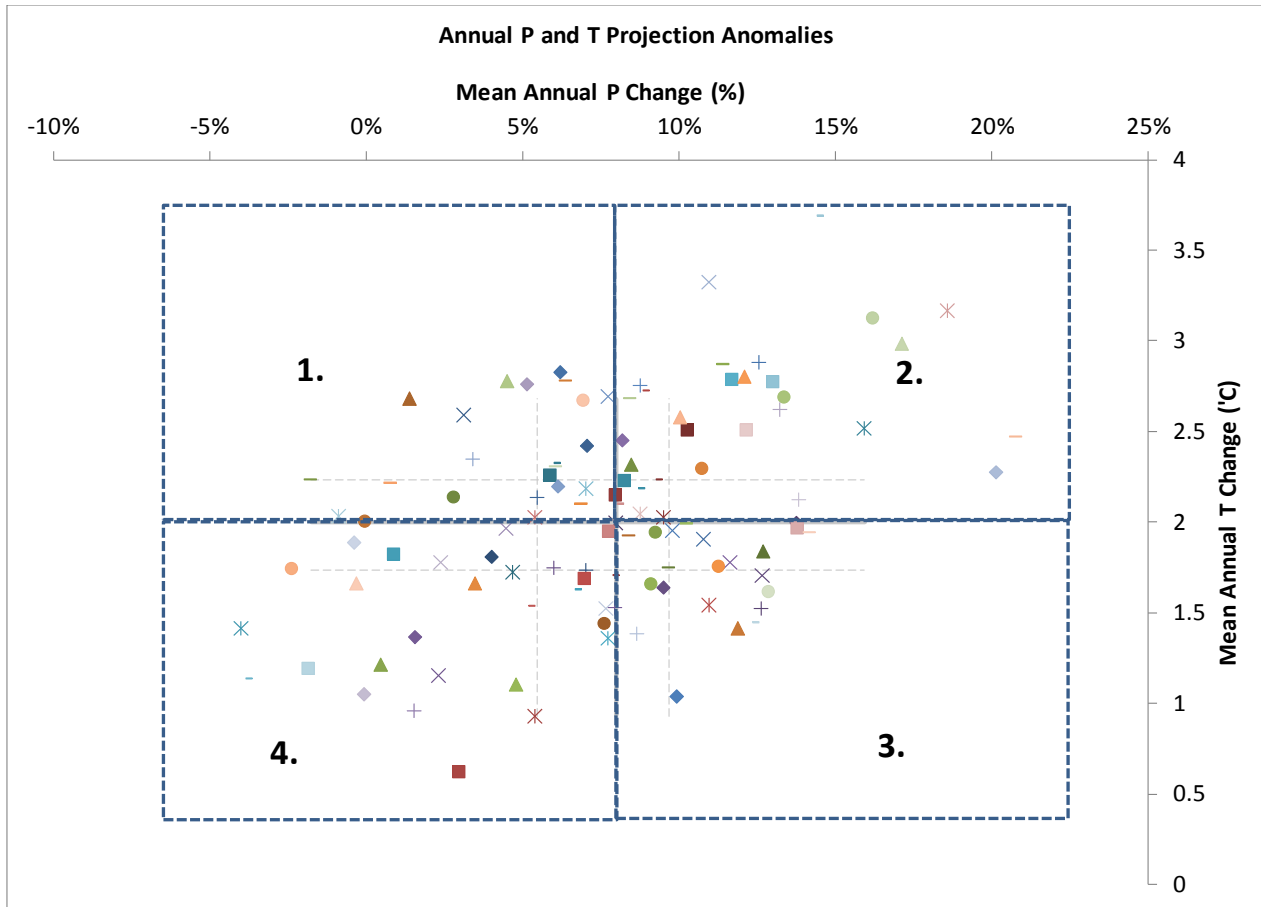
Figure 3-21. Annual Anomalies (2040 vs. historical) of GCM Temperature and Precipitation Projections, with Designated Scenario Ensembles (each symbol represents a different climate model projection set)
