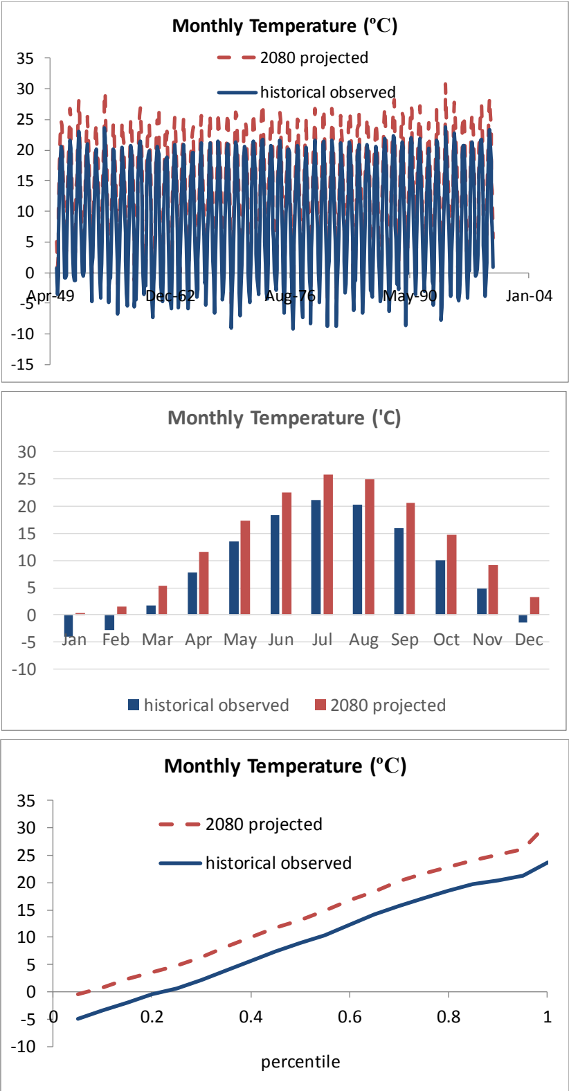
Figure 3-11. Monthly Temperature Projections: 2080 Planning Horizon, Hot Dry Ensemble
