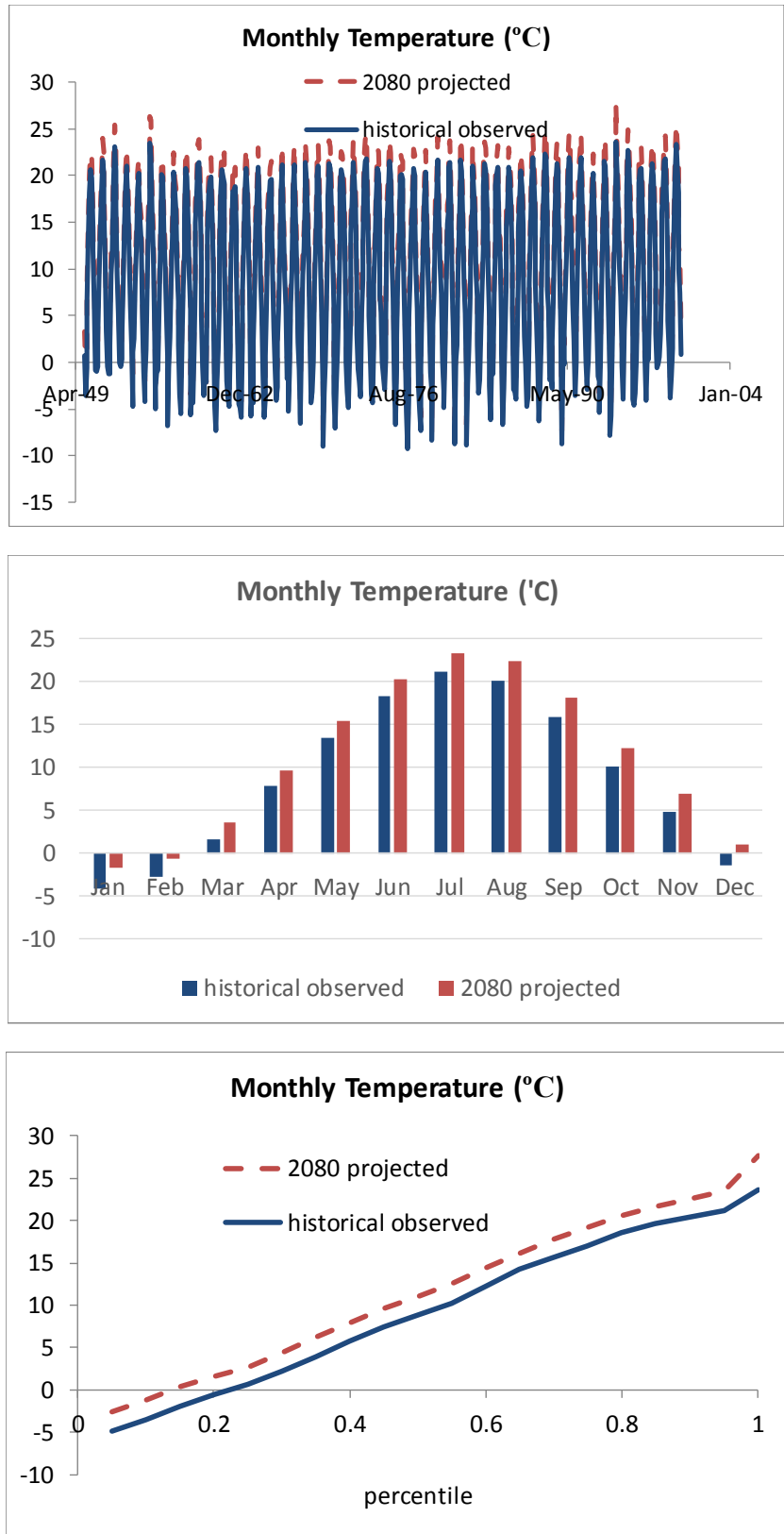
Figure 3-13. Monthly Temperature Projections: 2080 Planning Horizon, Warm Dry Ensemble
