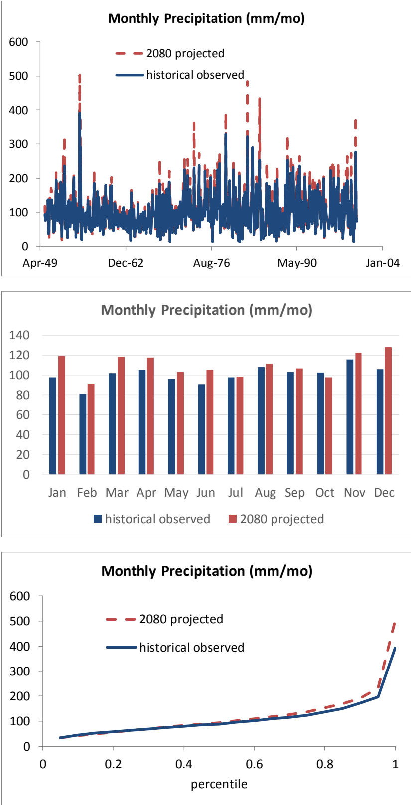
Figure 3-12. Monthly Precipitation Projections: 2080 Planning Horizon, Hot Dry Ensemble
