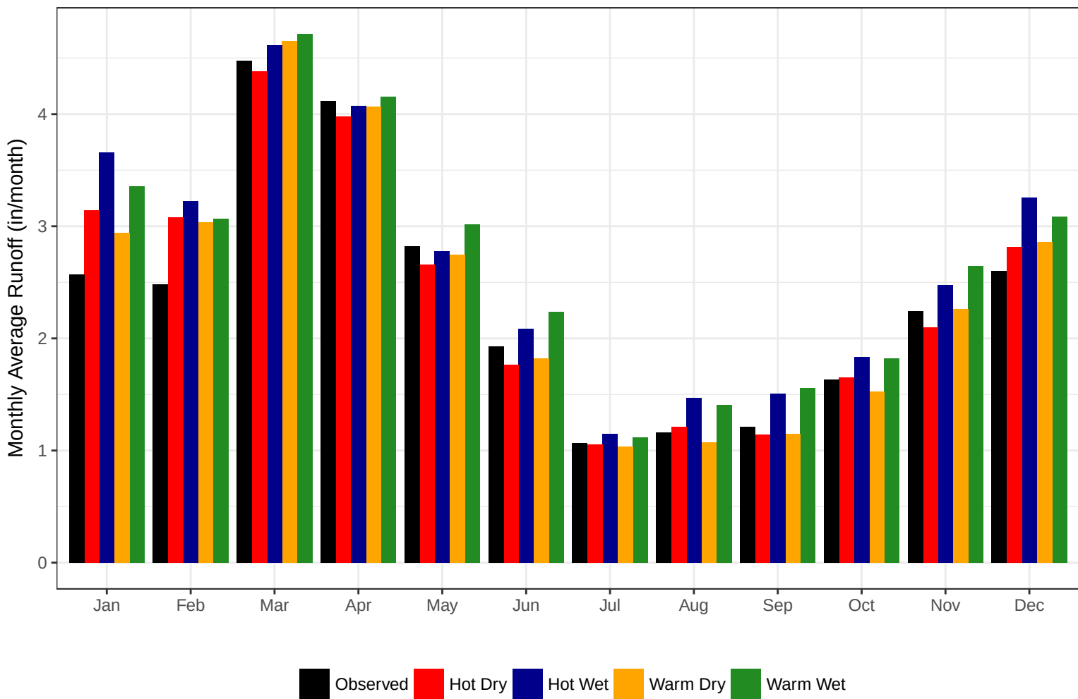
Climate Change Streamflow Projections for Park Regional Basin
