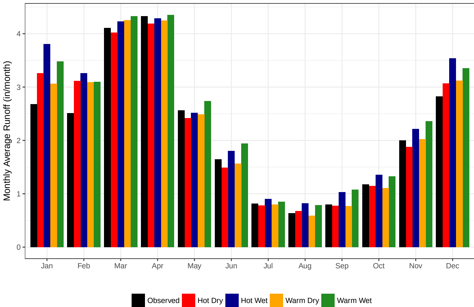
Climate Change Streamflow Projections for Housatonic Main Stem Regional Basin
