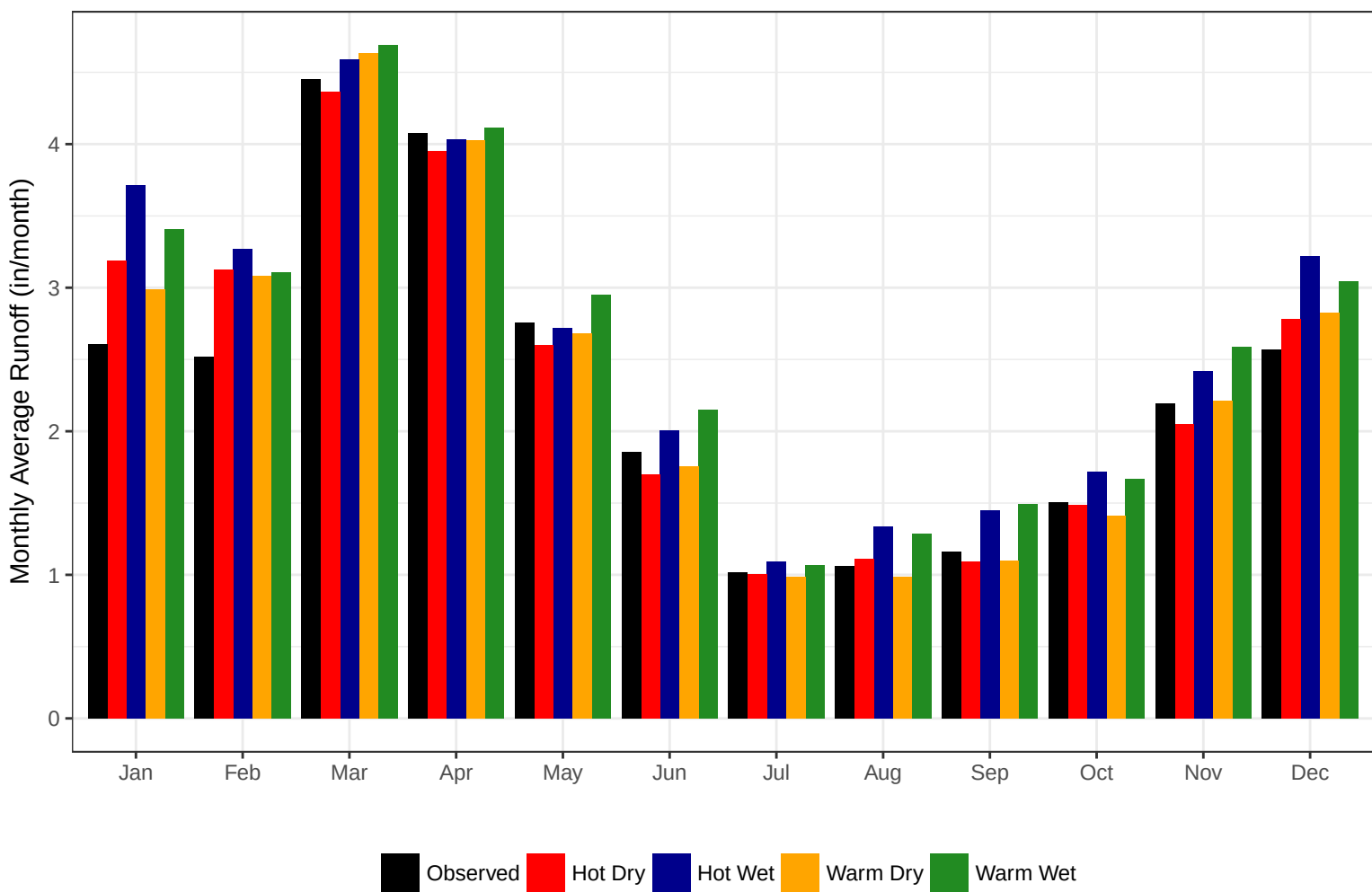
Climate Change Streamflow Projections for Naugatuck Regional Basin
